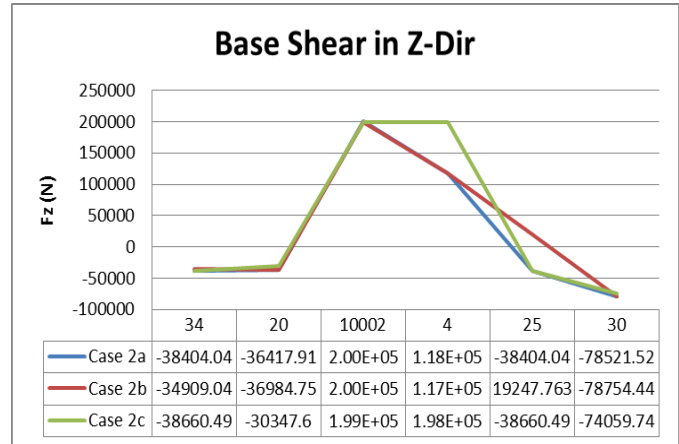
No. Of Nodes Vs Base Shear in Z Direction
