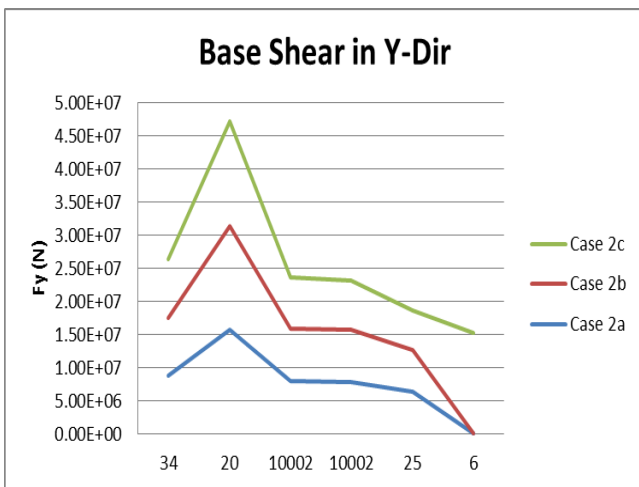
No. Of Nodes Vs Base Shear in Y Direction
