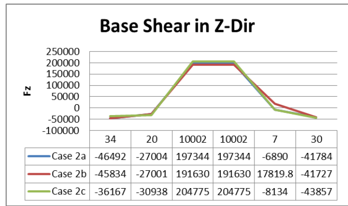
No. Of Nodes Vs Base Shear in Z Direction
