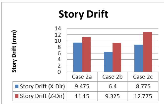
Story Drift in X & Z Direction
