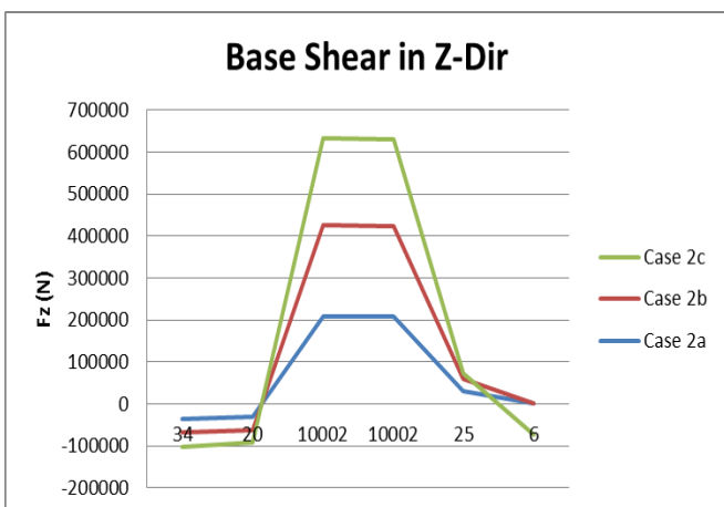
No. Of Nodes Vs Base Shear in Z Direction Story Drift in X & Z Direction
