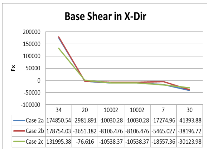
No. Of Nodes Vs Base Shear in X Direction
