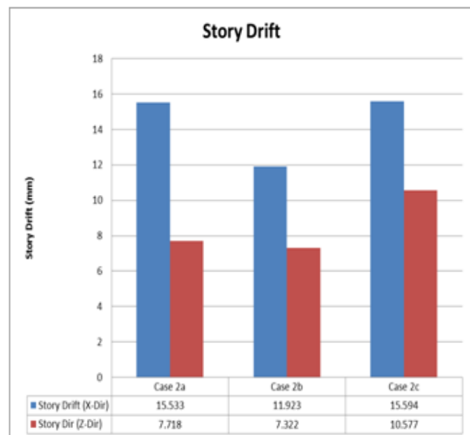
Story Drift in X & Z Direction
