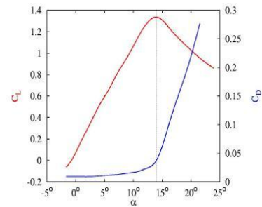
Figure 3: Relationship of Different Coefficients
