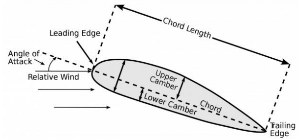
Figure 1: Basic nomenclature of an airfoil
