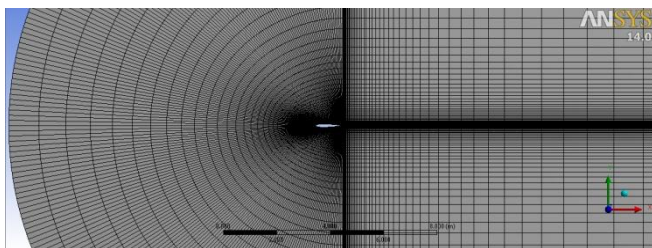
Figure 4 : meshed region
