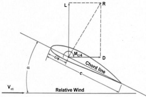
Figure 2: Angle of attack
