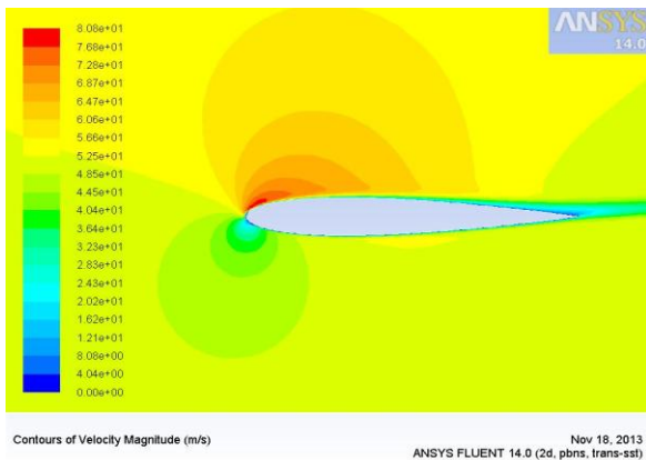
Figure 8: contours of velocity magnitude over NACA 0012 airfoil at 6 degree of AOA
