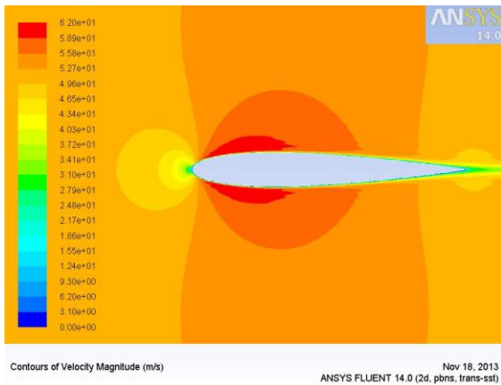
Figure 7: Contours of velocity magnitude over NACA 0012 airfoil at 0 degree of AOA
