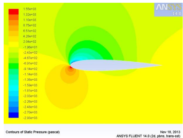
Figure 6: Contours of static pressure over NACA 0012 airfoil at 6 degree of AOA
