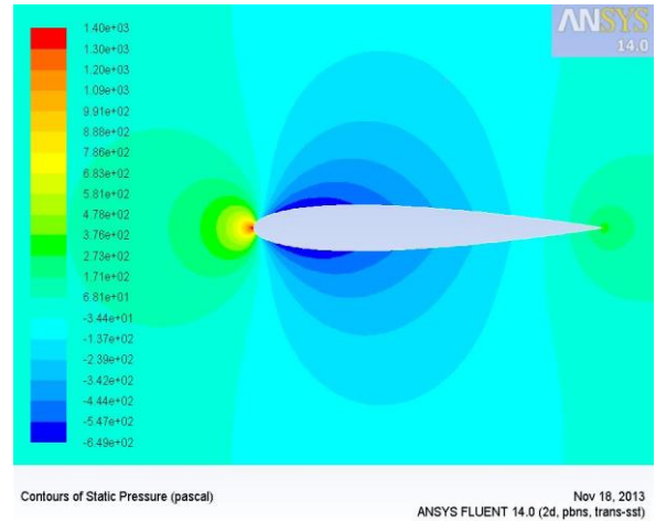
Figure 5: Contours of static pressure over NACA 0012 airfoil at 0 degree of AOA
