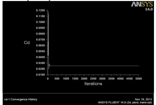
Figure 9: Graph of coefficient of drag at six degree of AOA.
